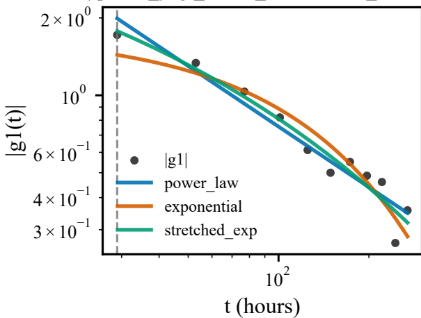
typhoon_yagi_across_northeastern_vietnam
