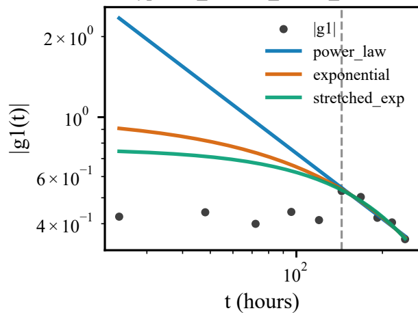
typhoon_krathon_across_taiwan
