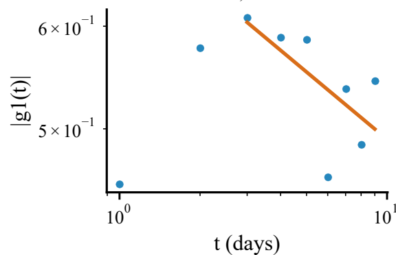
hurricane_milton_across_florida_us \alpha=0.17, R^2=0.42
