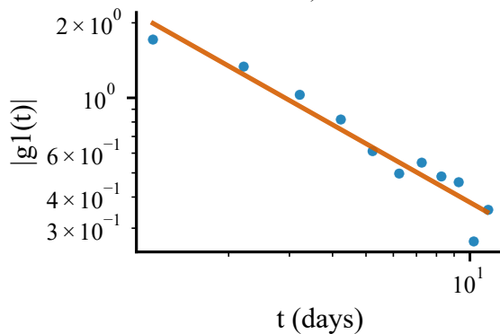
typhoon_yagi_across_northeastern_vietnam \alpha=0.78, R^2=0.93
