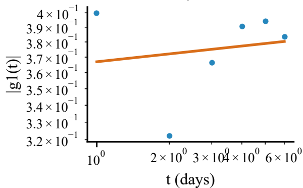
hurricane_john_across_southeastern_guerrero_mexico \alpha=-0.02, R^2=0.03
