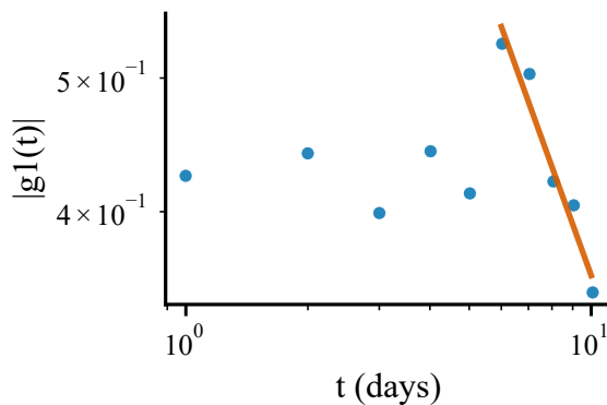
typhoon_krathon_across_taiwan \alpha=0.81, R^2=0.95
