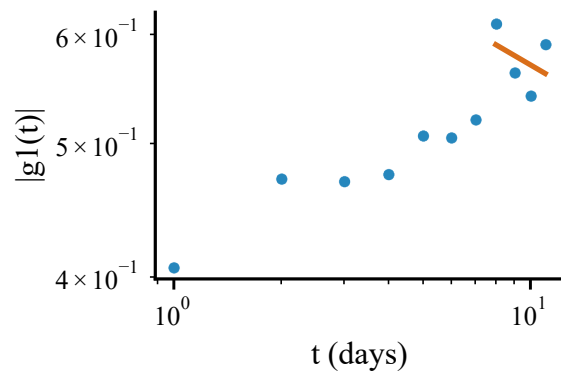
hurricane_helene_pre_landfall_gulf_of_mexico_24_septemb \alpha=0.15, R^2=0.16
