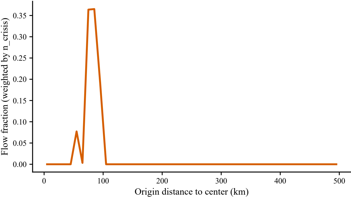
Origin distance histogram (hurricane_beryl_pre_landfall_2024)\nstart=50-100km, cos_alpha < 0 (inward
