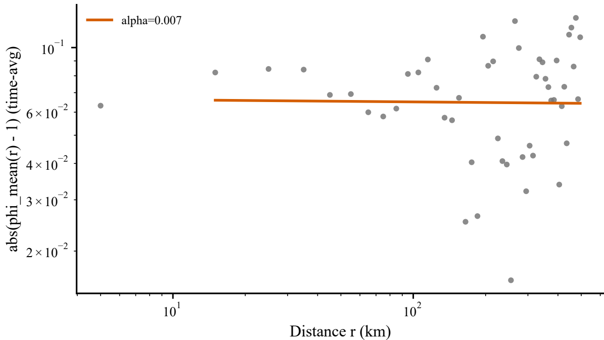
hurricane_john_southern_mexico_25_september_2024: power-law fit, t in [24.0,72.0]h
