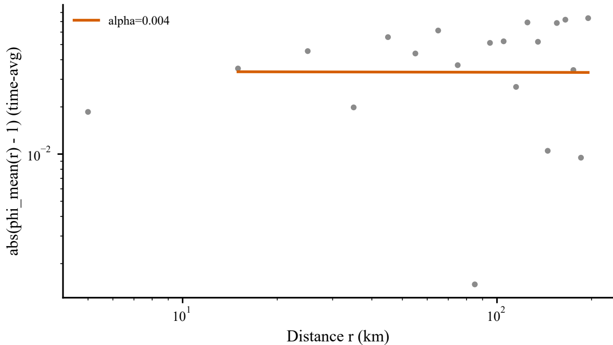
moldova_flooding_2024: power-law fit, t in [24.0,72.0]h
