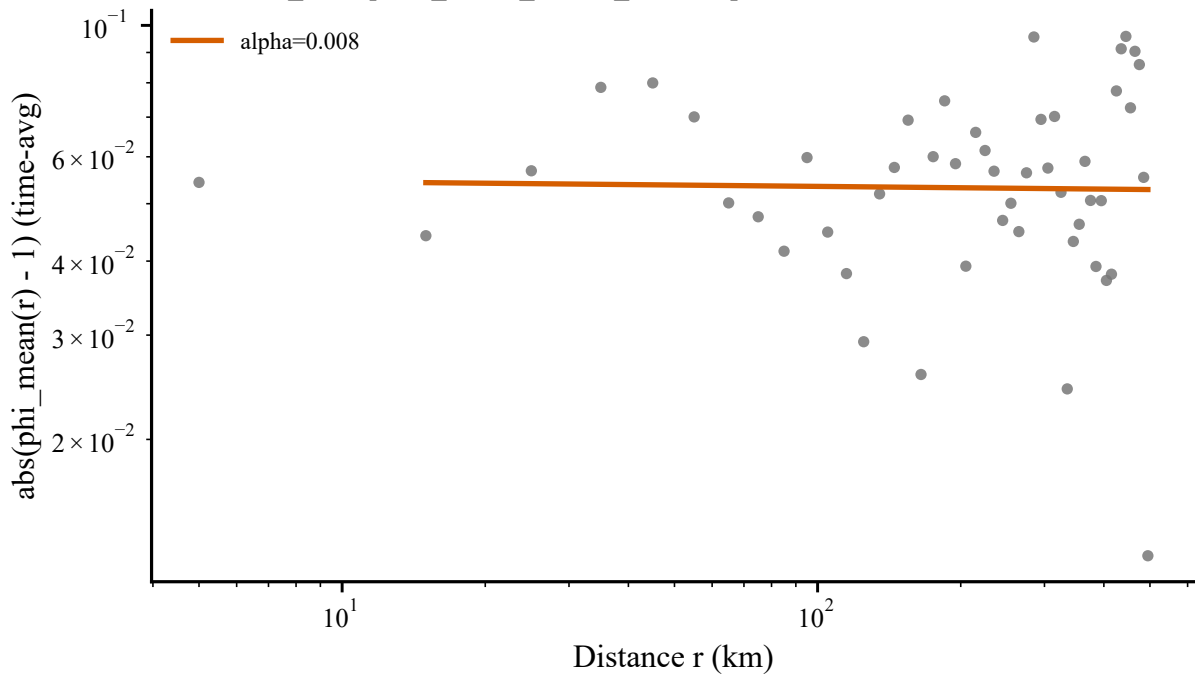
the_earthquake_across_central_mexico: power-law fit, t in [24.0,72.0]h
