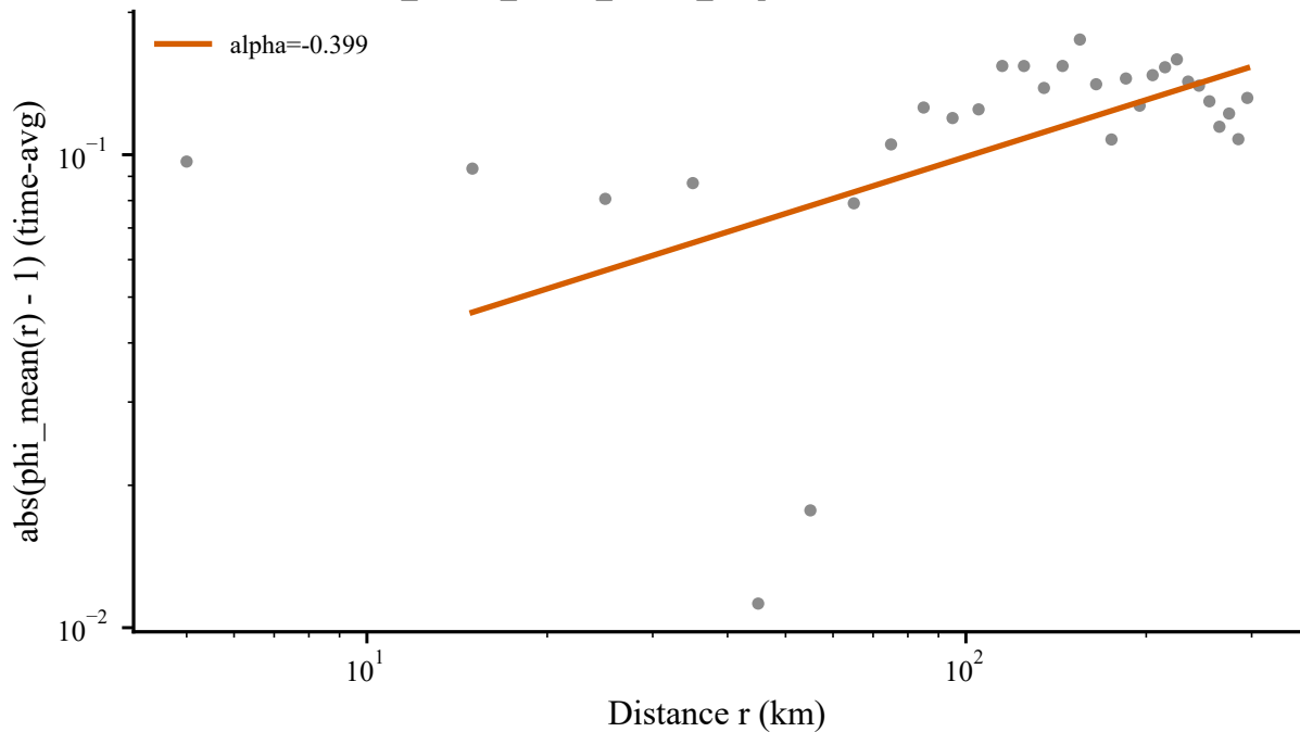
hurricane_milton_across_florida_us: power-law fit, t in [24.0,72.0]h
