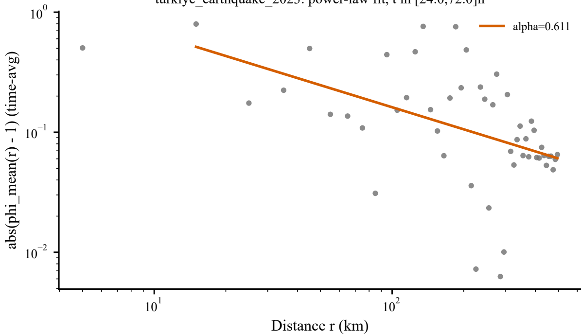
turkiye_earthquake_2023: power-law fit, t in [24.0,72.0]h
