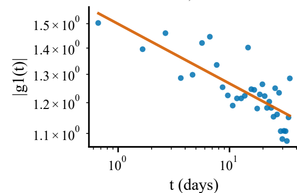
turkiye_earthquake_2023 \alpha=0.07 , R^2=0.63
