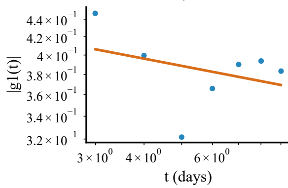
hurricane_john_across_southeastern_guerrero_mexico \alpha=0.09 , R^2=0.12
