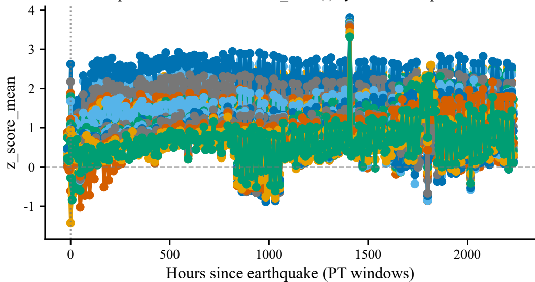
Population relaxation: mean z\_score(t) by distance to epicenter
