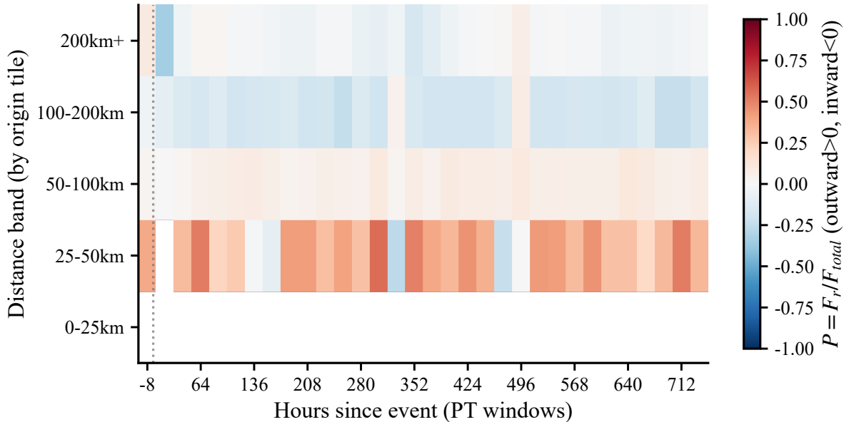
Directional polarization P(r, t) heatmap (hurricane_beryl_pre_landfall_2024)
