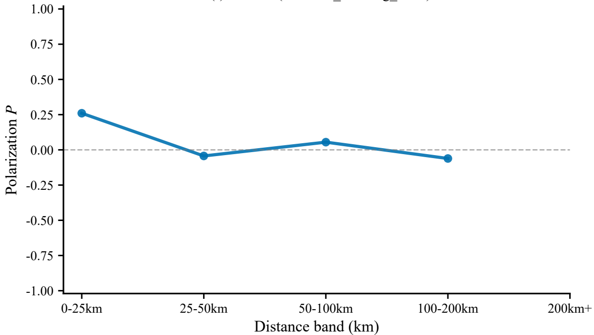
P(r) at t=-8h (moldova_flooding_2024)
