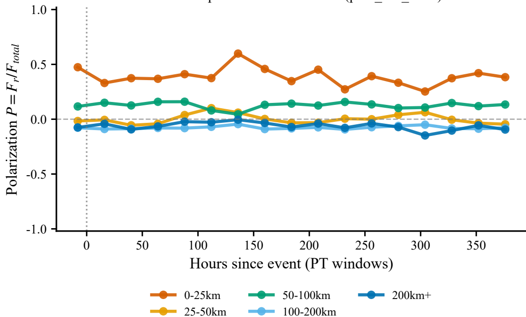
Directional polarization time series (park_fire_2024)
