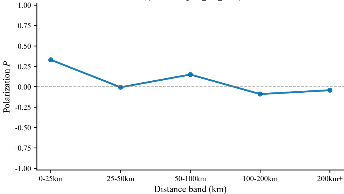
P(r) at t=16h (park_fire_2024)
