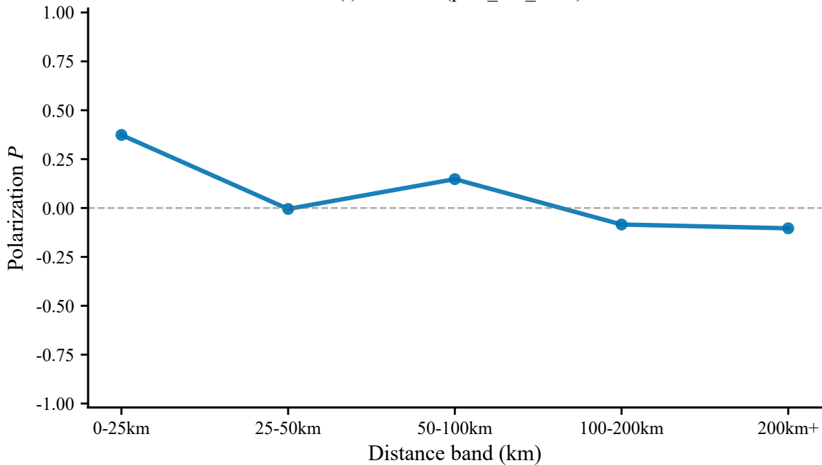
P(r) at t=328h (park_fire_2024)
