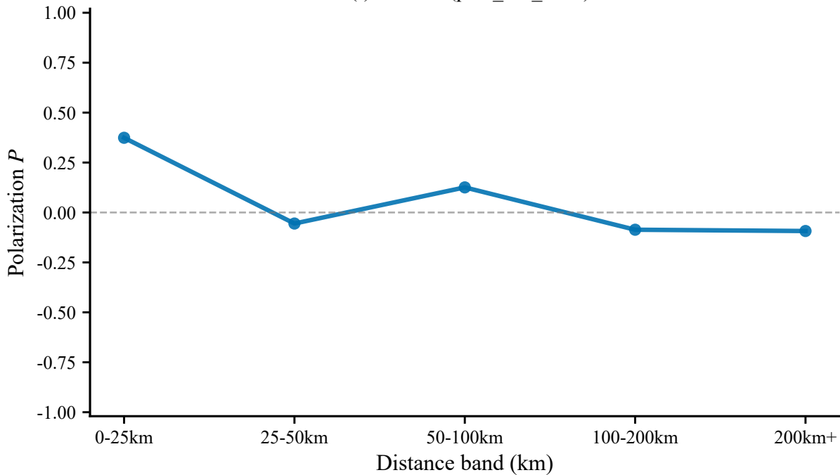
P(r) at t=40h (park_fire_2024)
