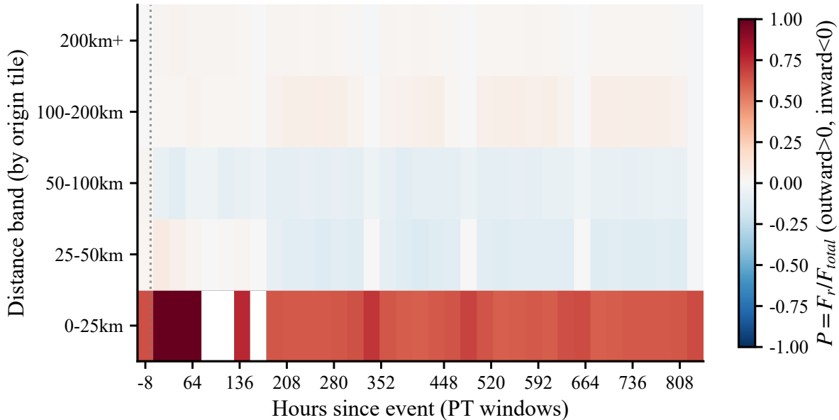
Directional polarization P(r, t) heatmap (turkiye_earthquake_2023)
