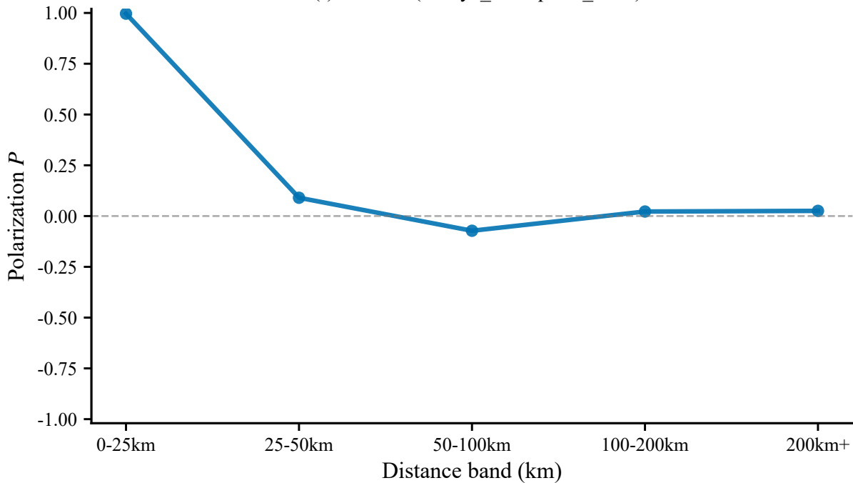
P(r) at t=16h (turkiye_earthquake_2023)
