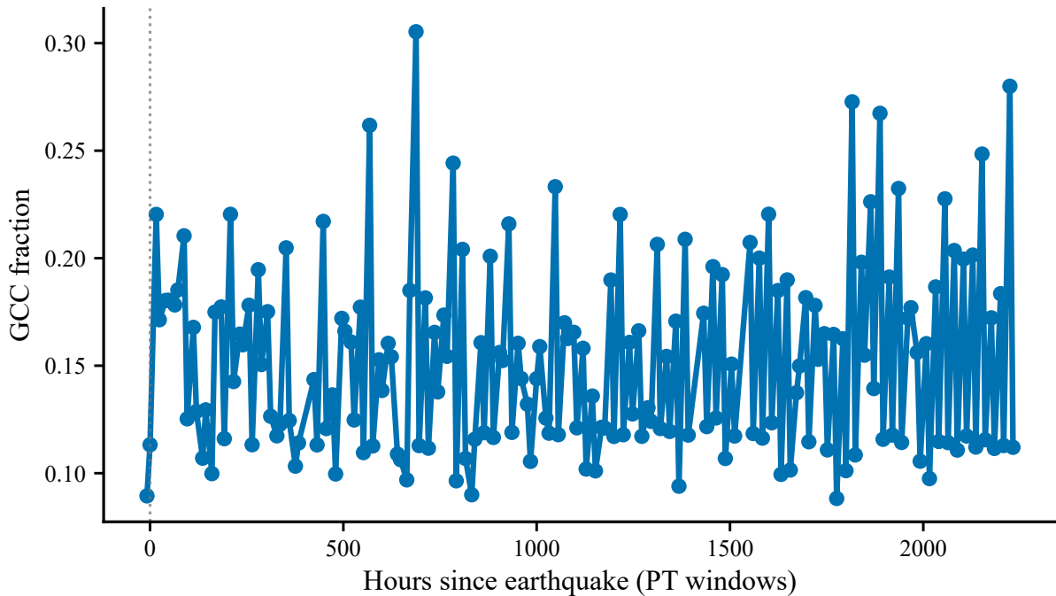
Movement network order parameter: GCC fraction over time
