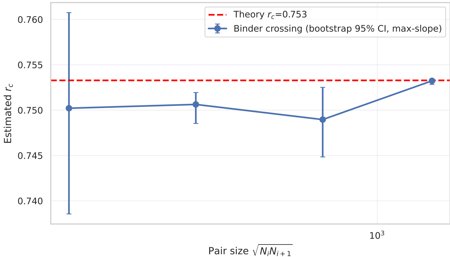
Finite-Size Scaling: r_c from Binder crossings
