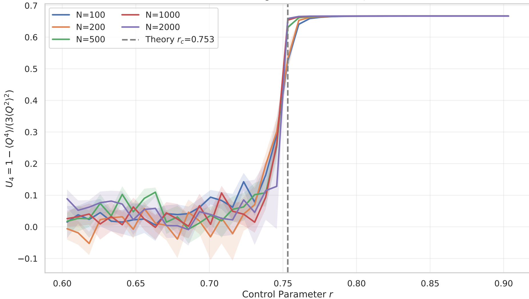
Finite-Size Scaling: Binder cumulant U_4(r; N)
