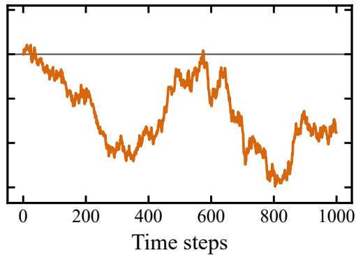
Near critical ( r=0.73 )
