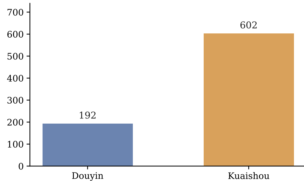
Edges
