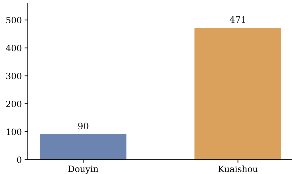
Nodes
