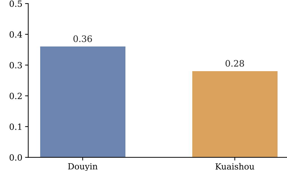
Clustering coefficient
