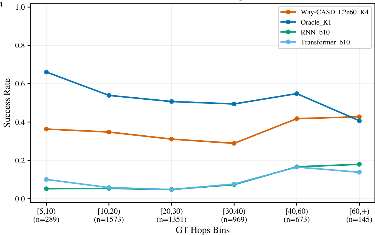
Success Rate vs GT Hops
