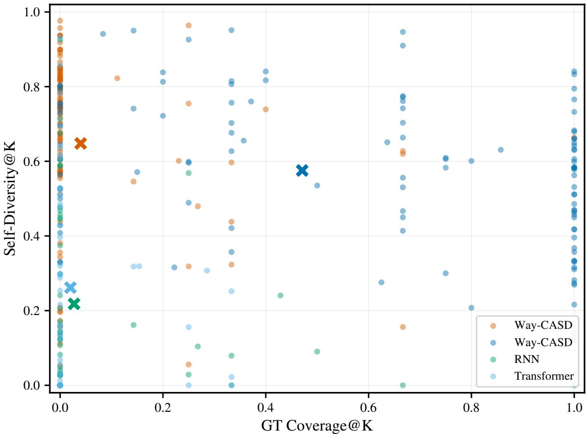
OD-level GT Coverage vs Self-Diversity (K=16)
