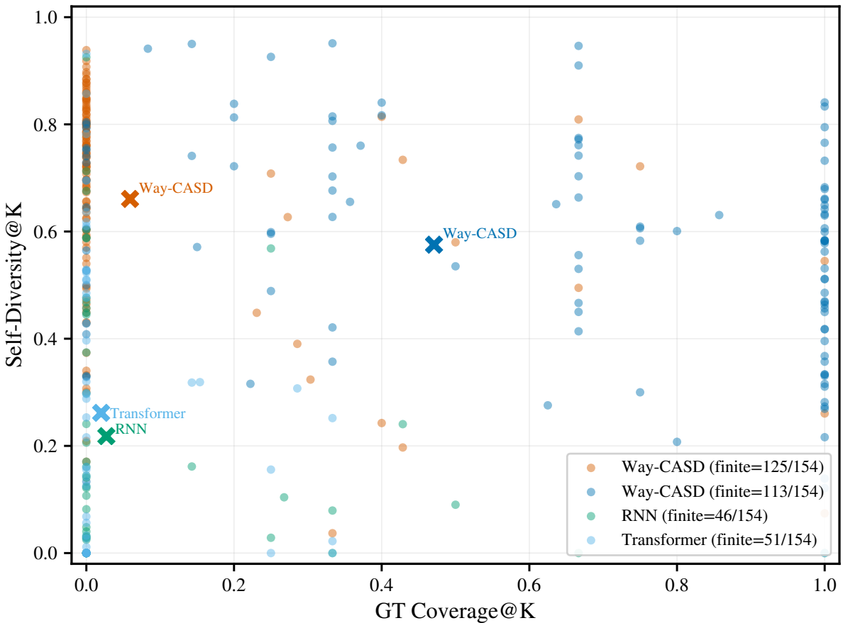
OD Coverage vs Diversity (Porto, K=16)
