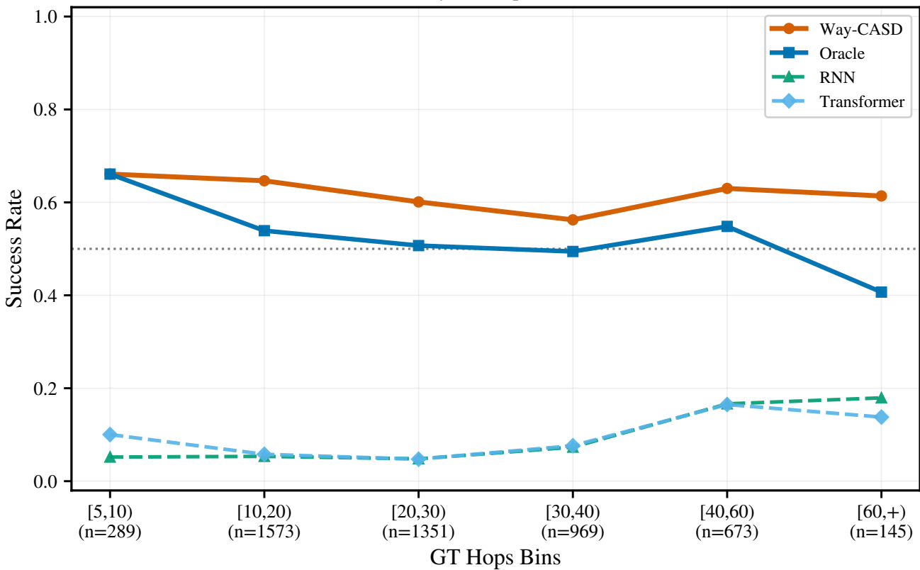
Success Rate by GT Hops (K=16, n=5000)
