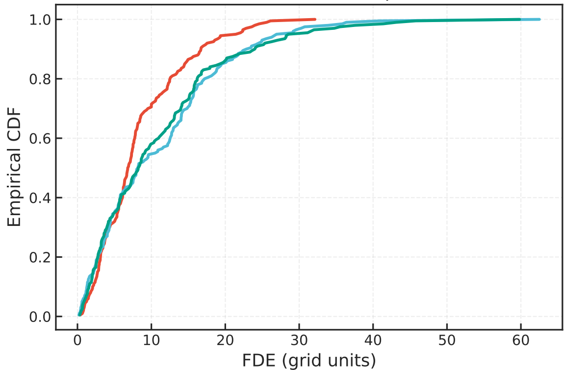
FDE CDF (saved samples)
