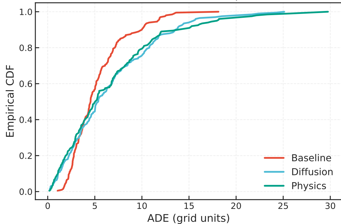
ADE CDF (saved samples)
