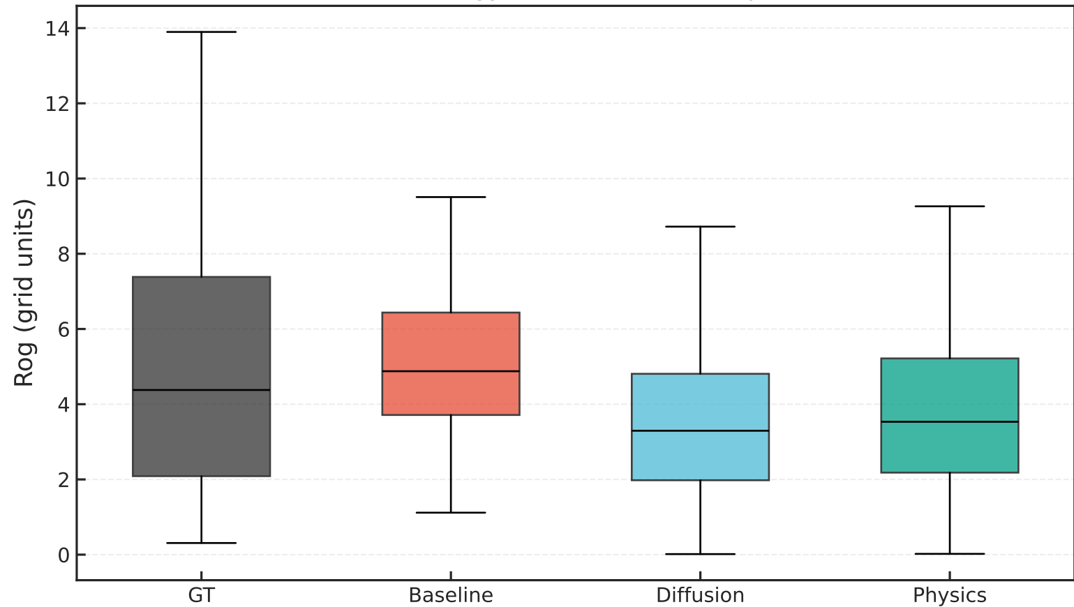
Radius of gyration (saved samples)
