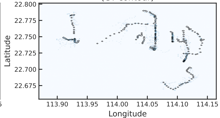
Diffusion: Pred density (GT contour)
