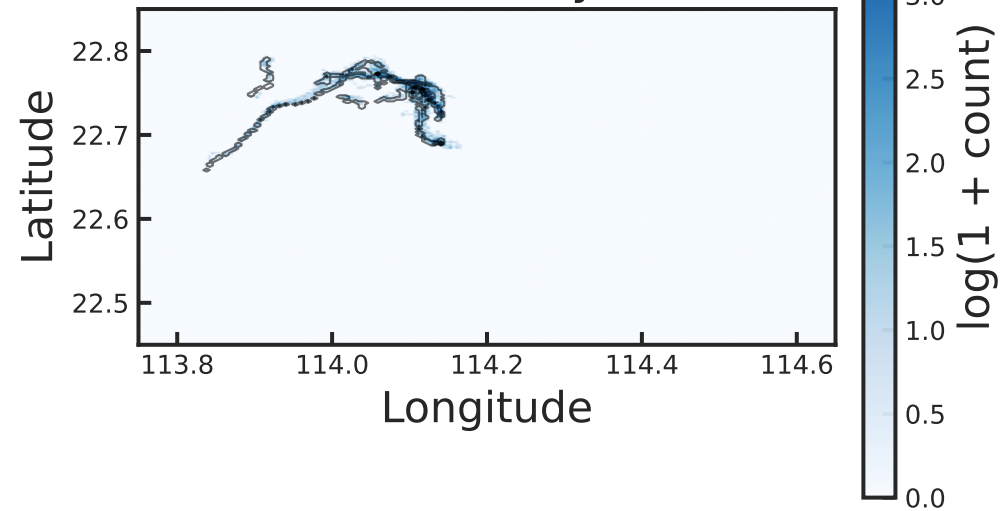
Diffusion: Pred density (GT contour)
