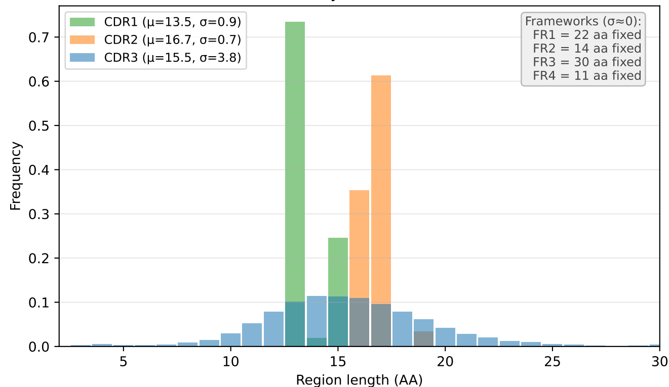
Heavy chain (VH)
