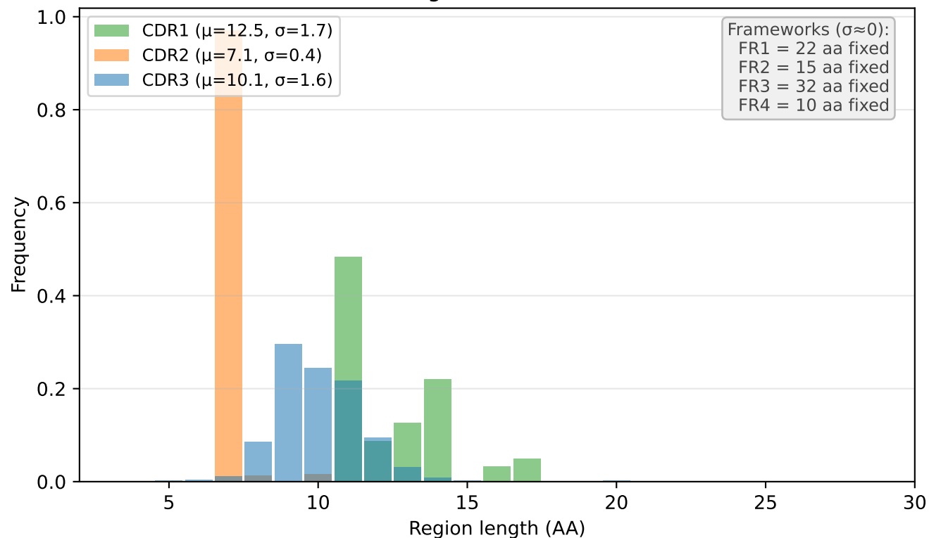
Light chain (VL)
