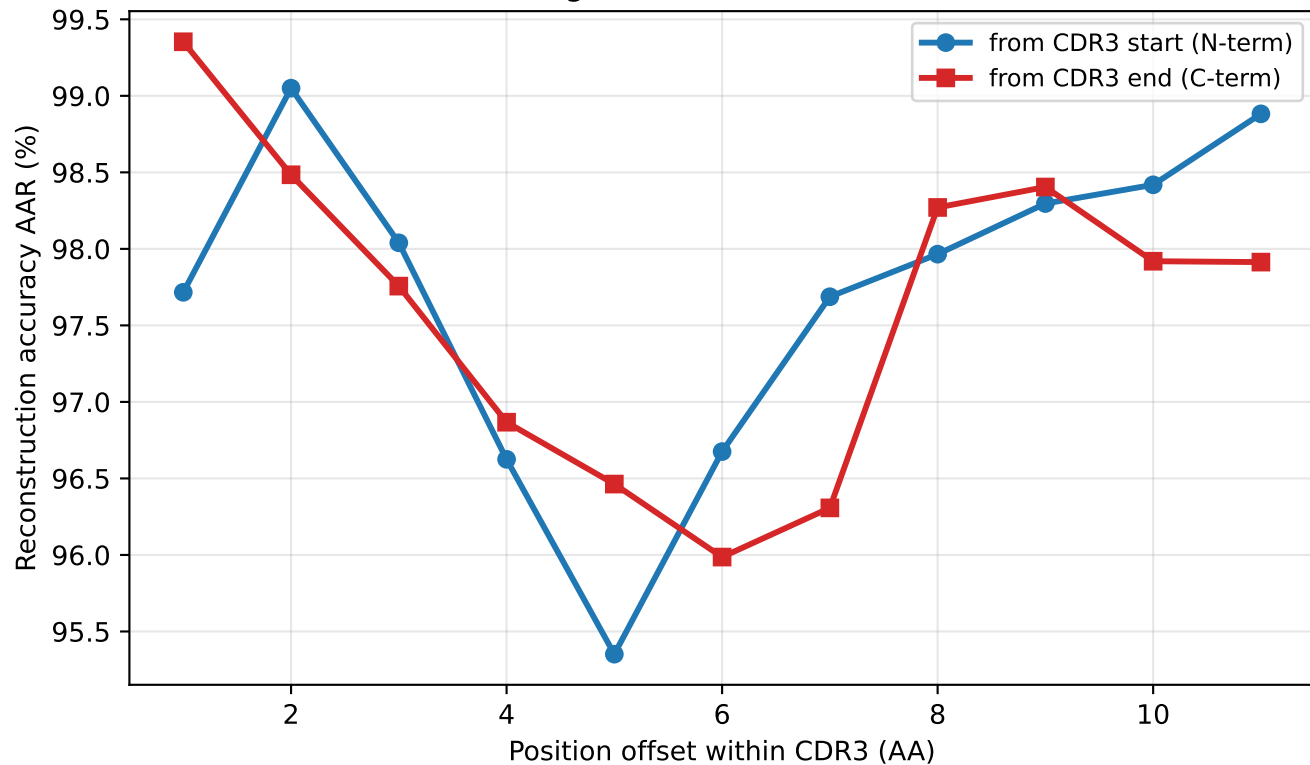
Light chain — VL CDR3
