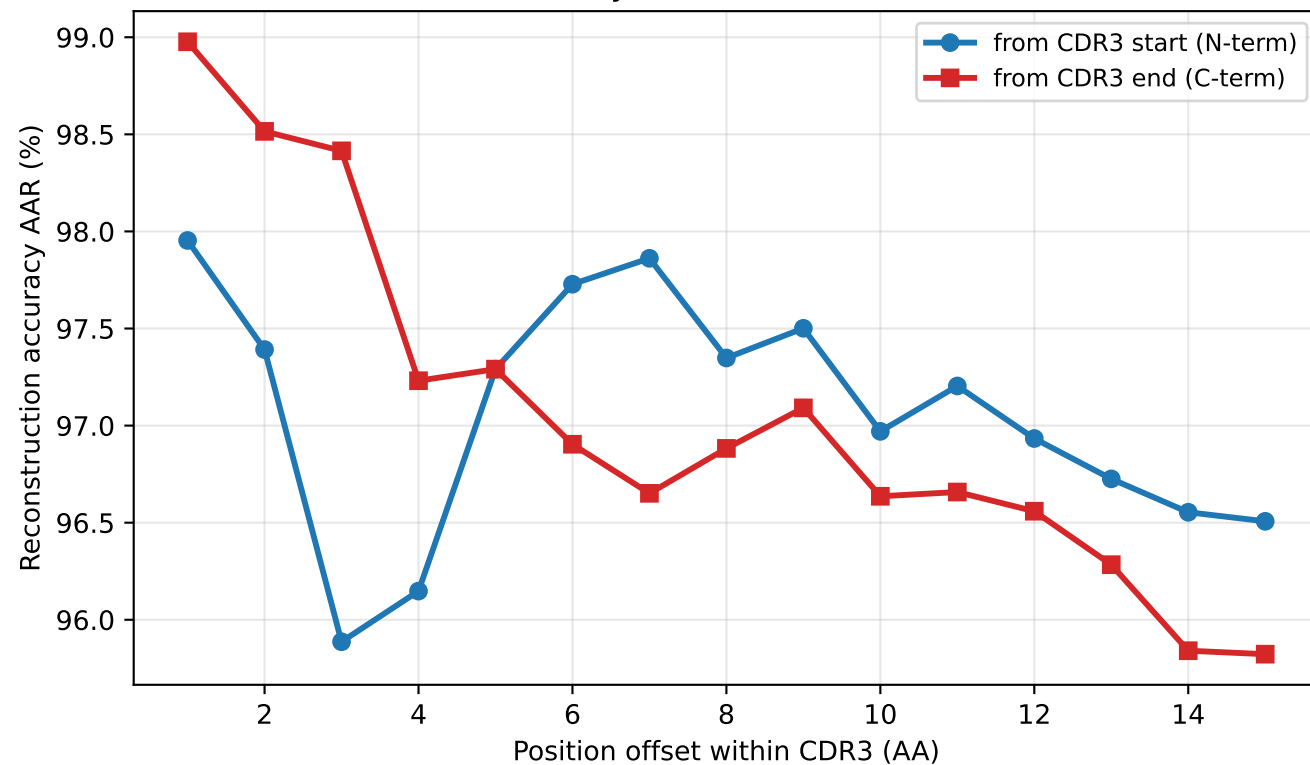
Heavy chain — VH CDR3
