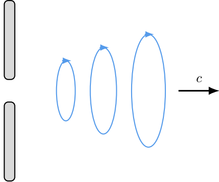
(b) beyond \sim \lambda/2\pi : the loops close on themselves and leave - no metal anywhere
