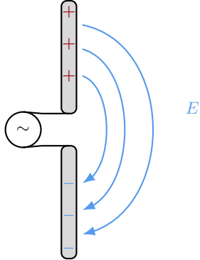
(a) near field: the lines end on the metal, and the energy comes back
