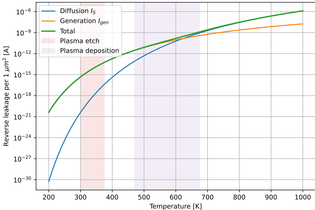
n+/p-well antenna ndiode, V_R = 1 V, per 1\ \mu\text{m}^2 , 200-1000 K
