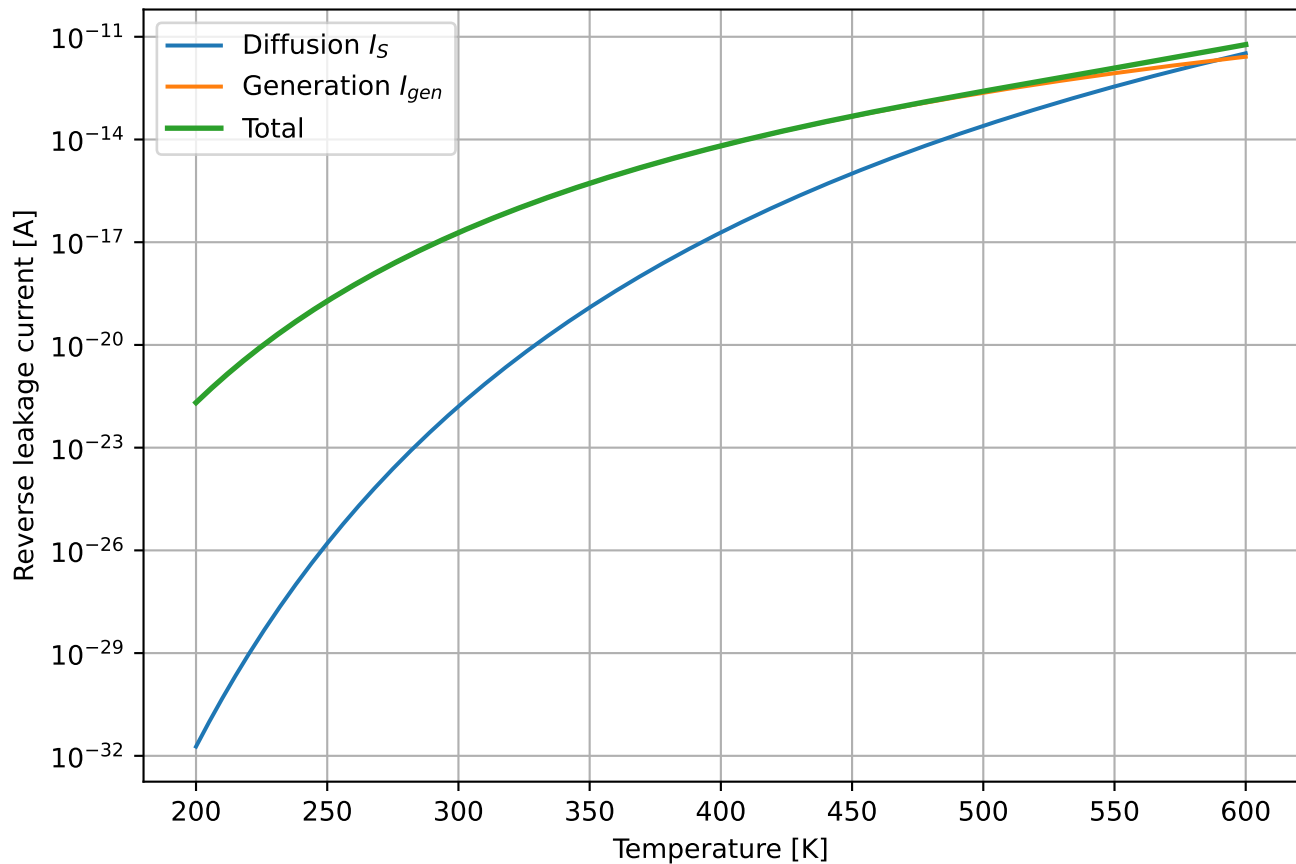
0.2×0.2 \mu\text{m}^2 antenna ndiode (n+/p-sub), V_R = 1 V
