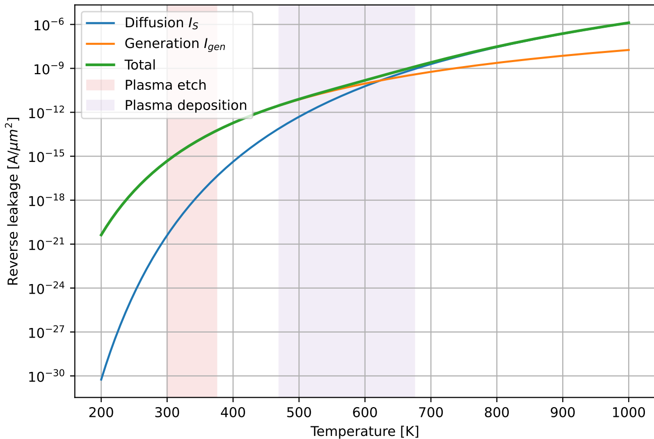
n+/p-well antenna ndiode, V_R = 1 V, 200-1000 K
