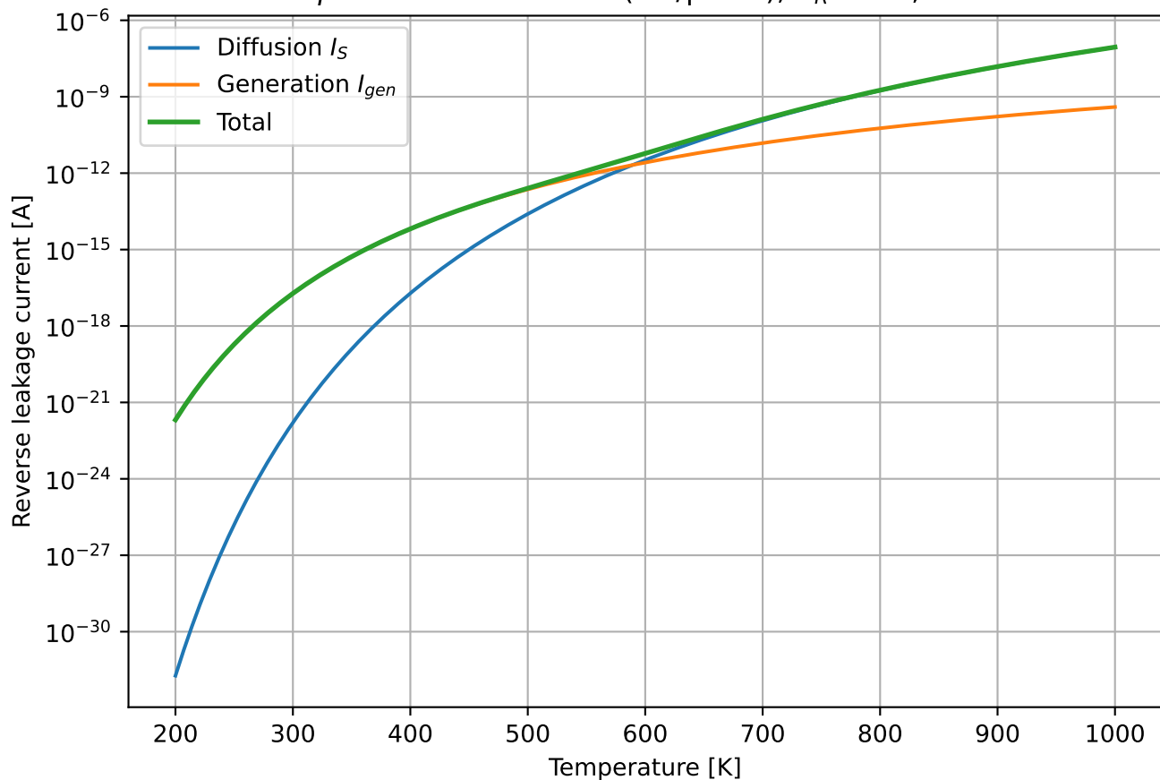
0.2 \times 0.2 \mu\text{m}^2 antenna ndiode (n+/p-sub), V_R = 1 \text{ V} , 200-1000 K
