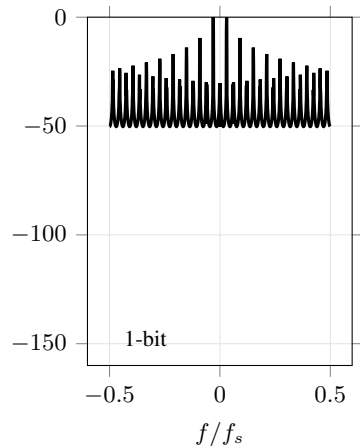
Discrete time, discrete value
