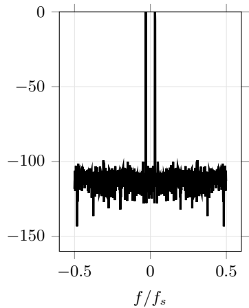
Discrete time, continuous value
