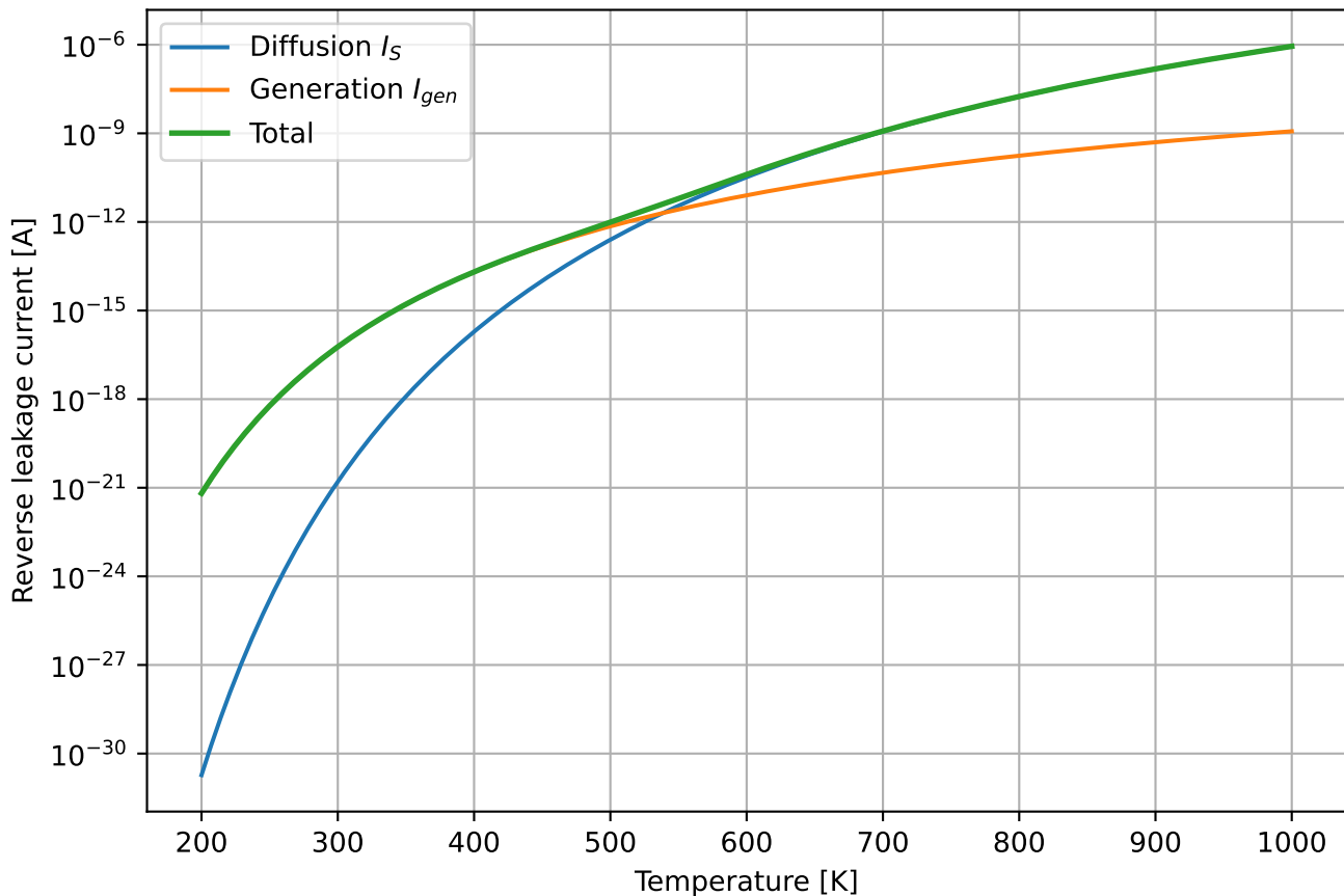
0.2×0.2 \mu\text{m}^2 antenna ndiode (n+/p-sub), V_R = 1 V, 200-1000 K
