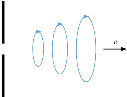
(b) beyond \sim \lambda/2\pi : the loops close on themselves - displacement current with no metal - and leave
