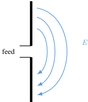
(a) near field: the field lines end on the metal, and the energy comes back
