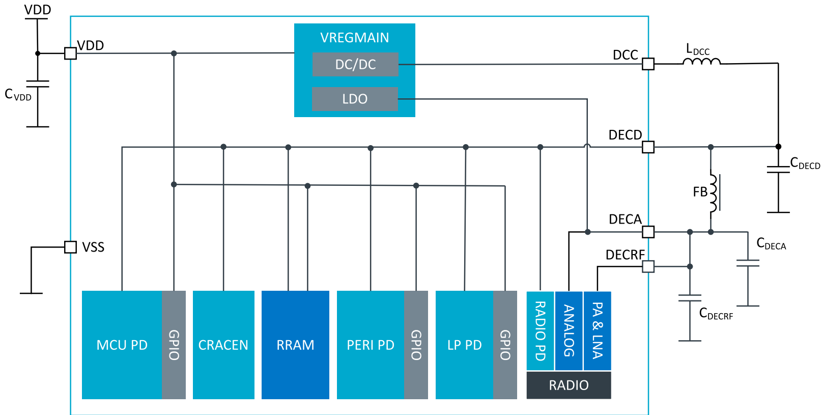
Figure 21: Regulator configuration
