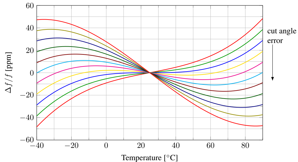
Temperature behaviour for AT cut crystals
