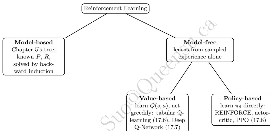
Figure 19.2: A map of the reinforcement learning methods this chapter develops.
