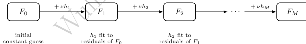
Figure 6.8: Gradient boosting as a sequential chain of shrunken trees, each fit to correct the previous stage's residuals.
