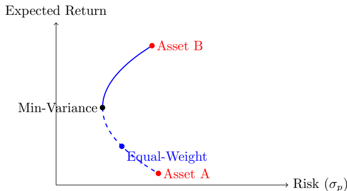
Figure 1.1: A schematic efficient frontier for the two-asset example (solid: efficient; dashed: feasible but dominated).
