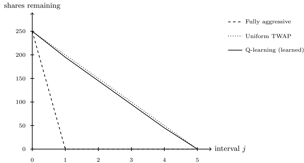
Figure 1.5: Unexecuted-share trajectories under the three strategies of Table ??.
