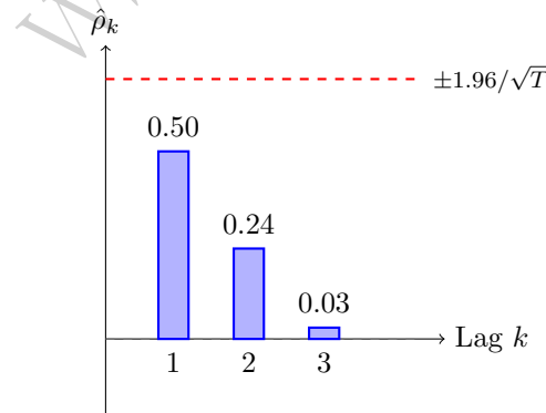
Figure 1.1: Sample correlogram for the interest-rate deviation series in Table ??, with the approximate 95% significance band \pm 1.96/\sqrt{T} (dashed red; symmetric about zero, so only its positive side is drawn).
