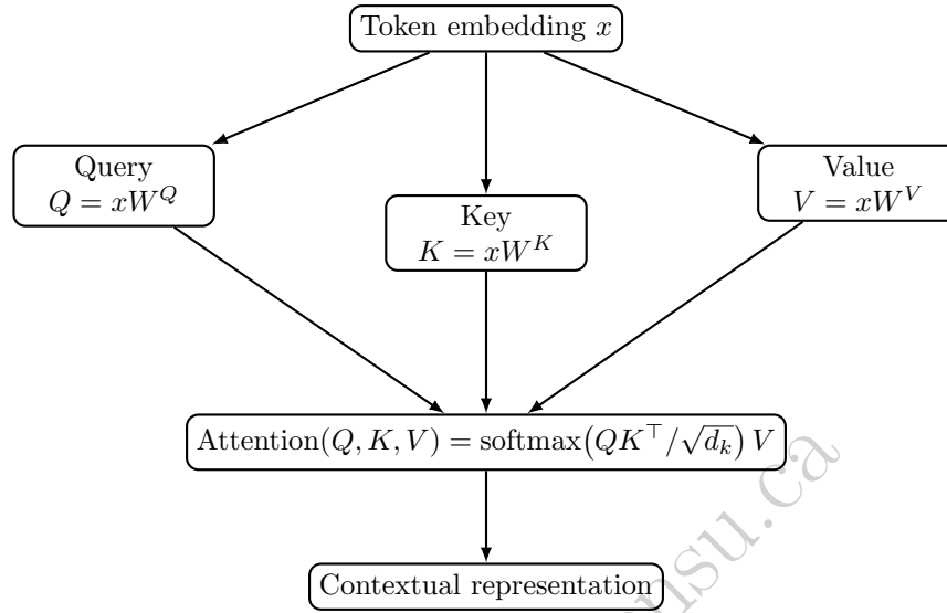
Figure 1.2: The self-attention computation as a diagram. The same token embedding x is projected three ways through independently learned weight matrices W^Q , W^K , W^V ; the resulting query, key, and value vectors are then combined by the attention formula into a single contextual representation.
