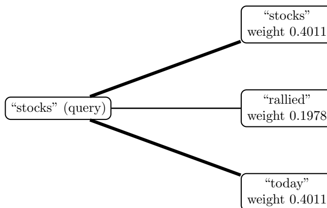
Figure 1.3: Self-attention weights for the query token “stocks” over the three-token sentence “stocks rallied today.” Edge thickness is proportional to attention weight: “stocks” and “today” each contribute about twice as much as “rallied” to the query token’s new, contextual representation, because their key vectors align more closely with the query.
