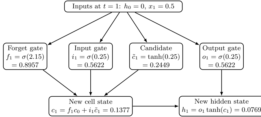
Figure 1.4: The LSTM cell’s first time step, computed from the worked example in the text. All four gates, forget, input, candidate, and output, are computed from the same inputs (h_0, x_1) ; the forget and input gates combine with the candidate value to produce the new cell state c_1 , and the output gate then determines how much of c_1 (passed through \tanh ) becomes the new hidden state h_1 .
