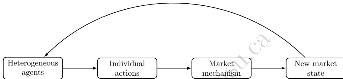
Figure 1.1: The basic agent-based simulation loop. Each agent observes the current market state and acts according to its own behavioral rule; a market mechanism (a double auction, a price-impact equation, a clearing algorithm) aggregates those individual actions into a new market state, which every agent then observes in the next round. Every example in this chapter is an instance of this loop with a different agent population and market mechanism.
